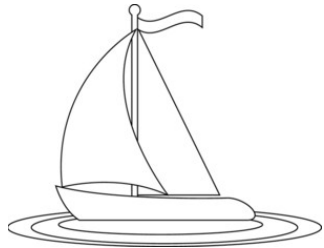
SAIL BOAT
